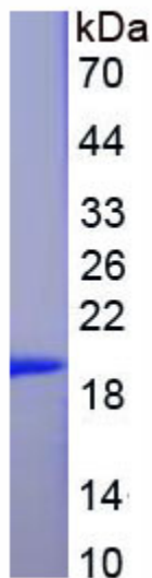
Figure. SDS-PAGE
