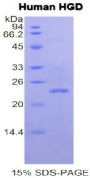
SDS-PAGE Image
