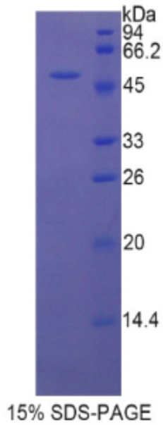
SDS-PAGE Image
