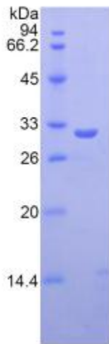
Figure. SDS-PAGE
