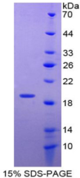
SDS-PAGE Image
