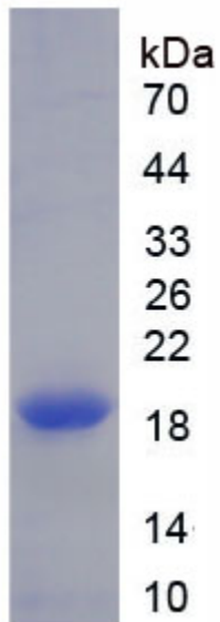
Figure. SDS-PAGE
