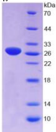
Figure. SDS-PAGE
