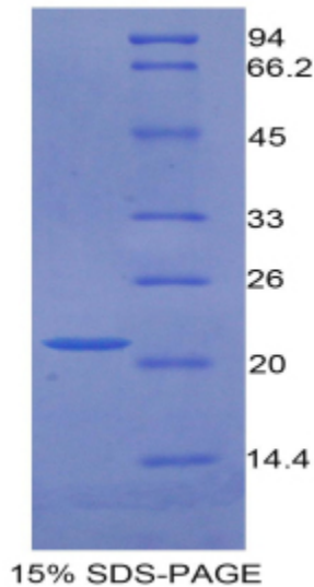
SDS-PAGE Image
