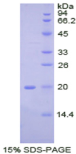
SDS-PAGE Image
