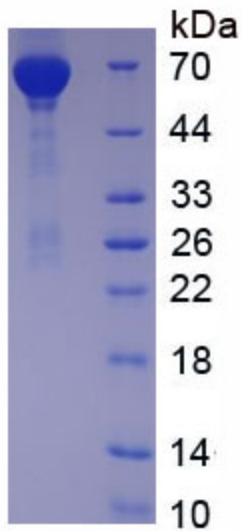
Figure. SDS-PAGE
