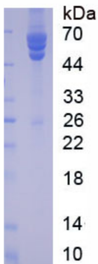
Figure. SDS-PAGE
