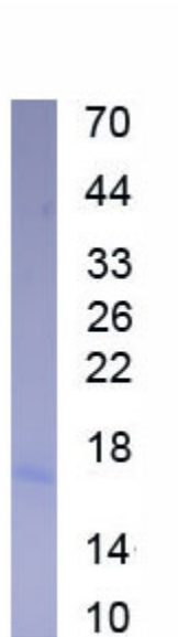
Figure. SDS-PAGE
