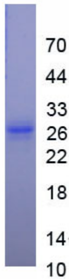
Figure. SDS-PAGE
