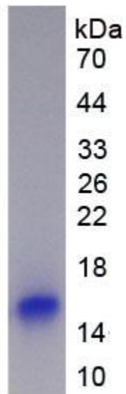
SDS-PAGE Image
