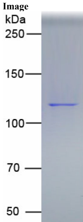
Figure. SDS-PAGE
