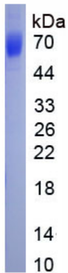
Figure. SDS-PAGE
