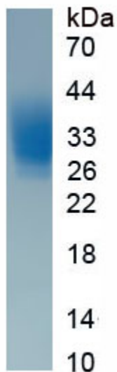
Figure. SDS-PAGE
