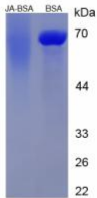
SDS-PAGE Image
