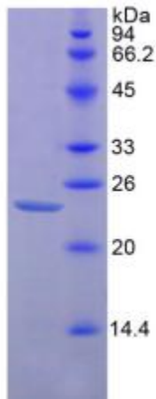
SDS-PAGE Image
